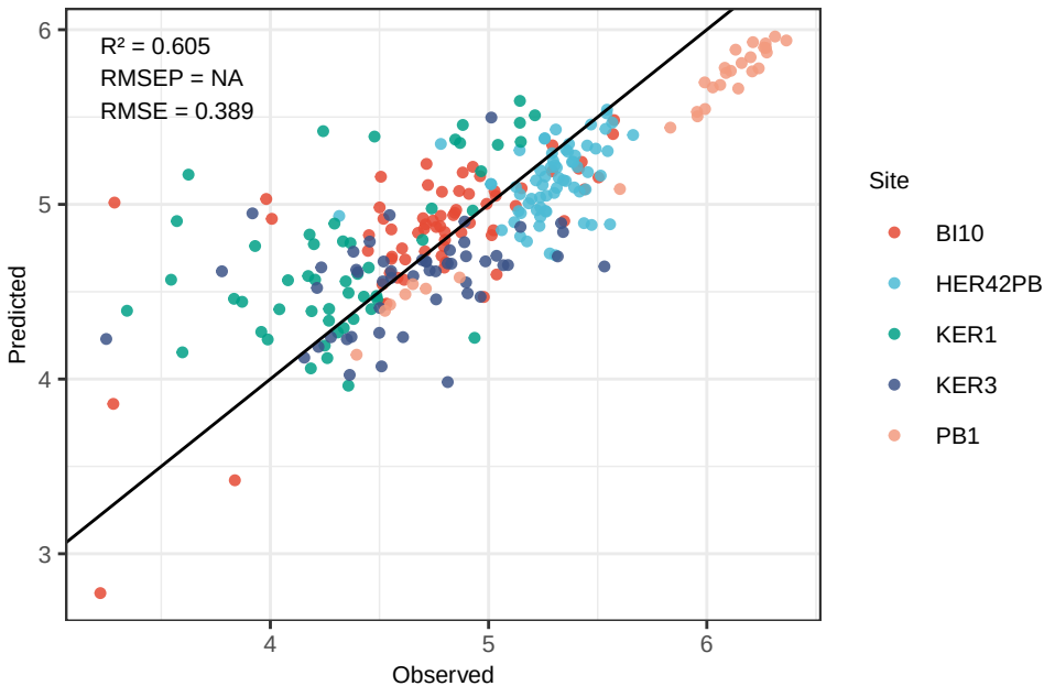
Sr WLS_weighted – Predicted vs Observed (log-space)
